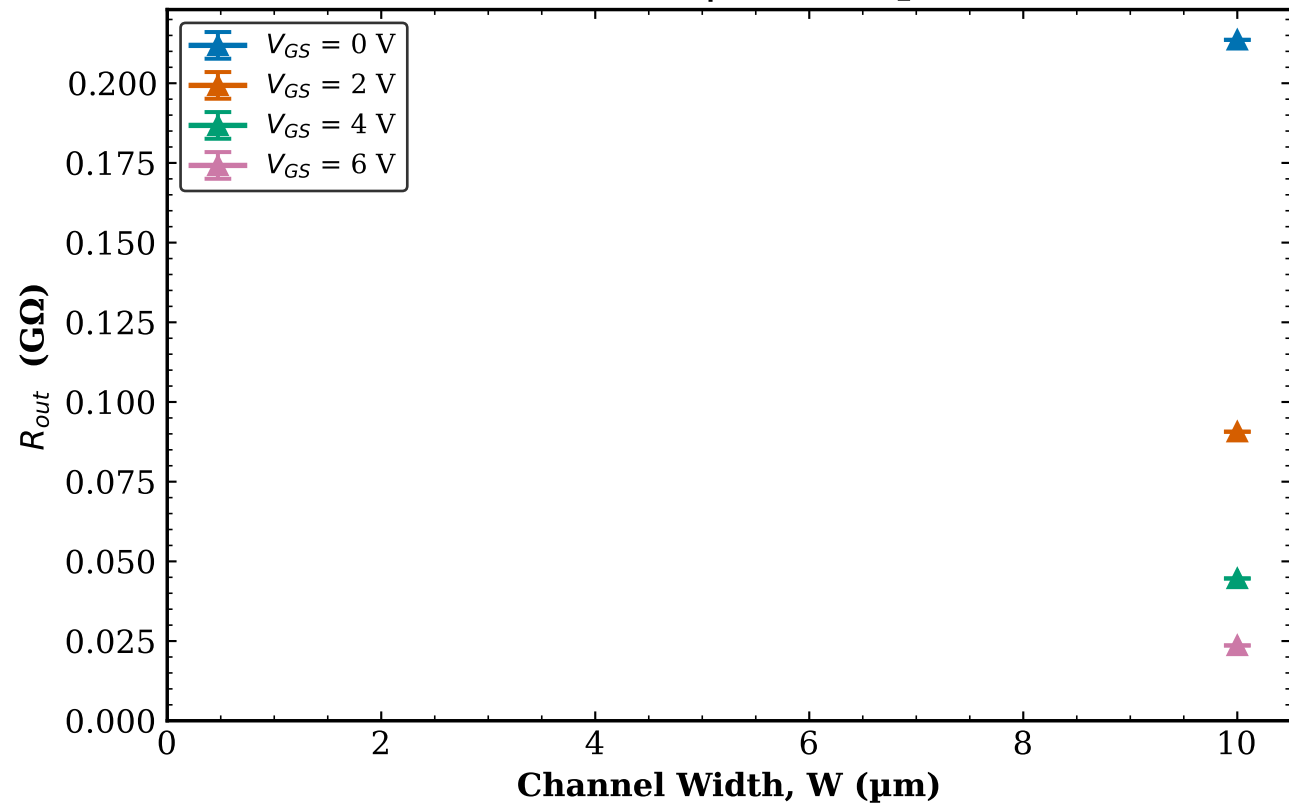
TFT3 Transistor 1 R_{out} vs W | L = 80\text{ }\mu\text{m}
